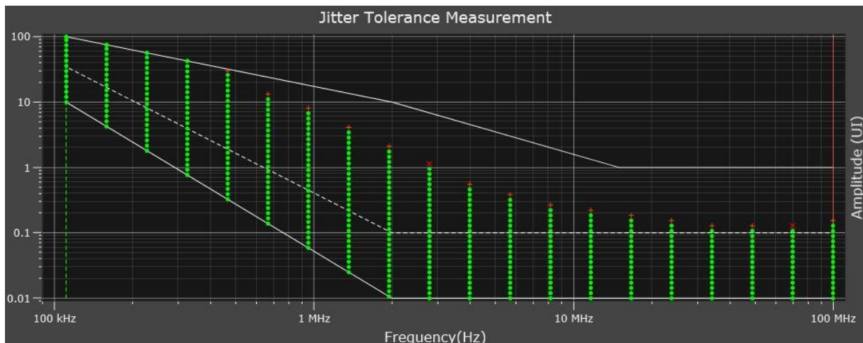
Figure 6. J-BERT M8020A provides automated jitter tolerance characterization and compliance measurements. A library of Jitter tolerance templates is available. To optimize test time, customized jitter tolerance templates can be created with a graphical jitter tolerance template editor. The red dots in the result screen show where the BER level was exceeded, the green dots show where the DUT tolerated the received jitter.
